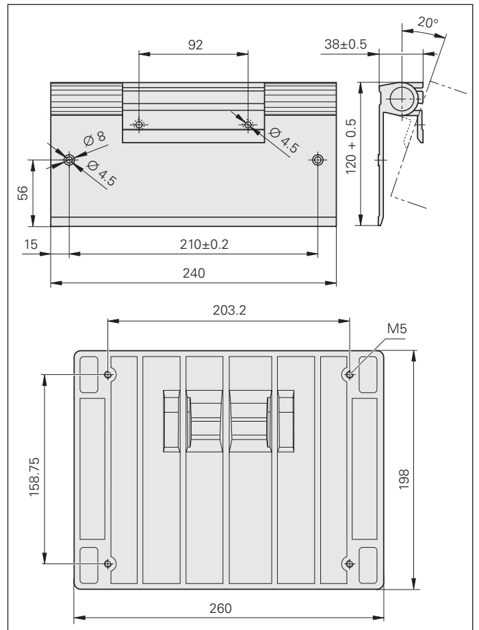
Tilting base for ND 780
