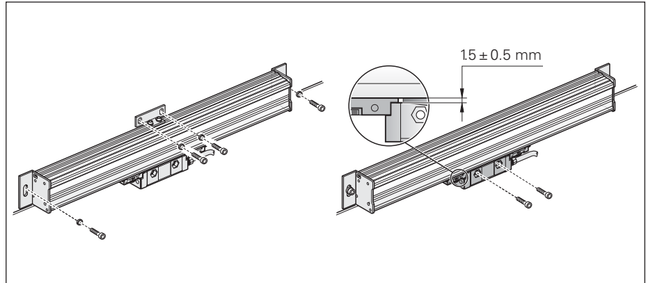
Mounting the LS 628C
